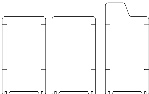
FLAT SHORT WRAP D 780MM x 1400MM FLAT SHORT END WRAP D2 780MM x 1400MM STEP UP WRAP E 780MM x 1650MM
