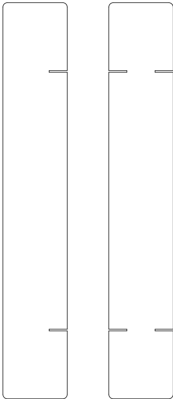
END PANEL PALING A
