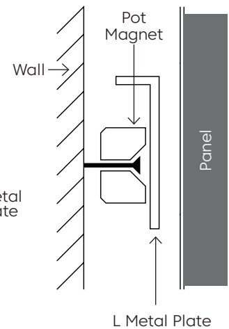
Wall Pot Magnet Install L Plate + Metal Plate
