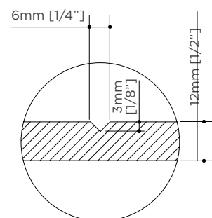
V-GROOVE DETAIL VIEW
